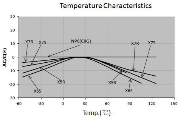
2、温度特性 Temperature Characteristics
