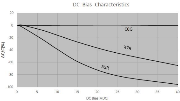
3、直流偏压特性 DC Bias Characteristics
